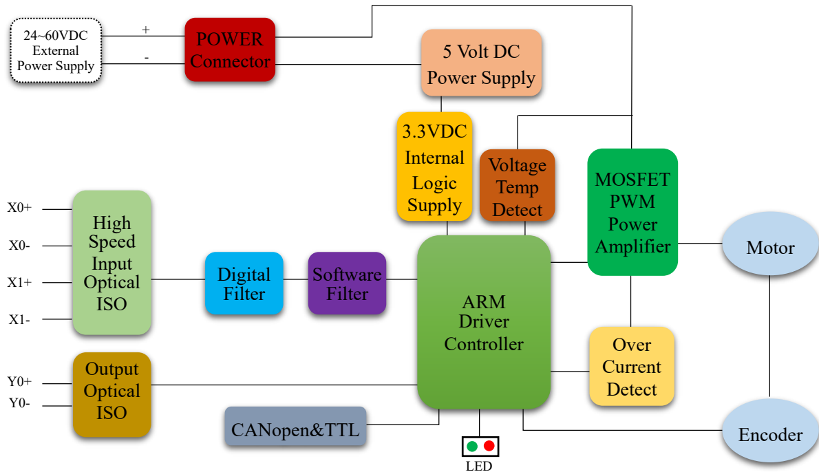
IR60EC Block Diagram
