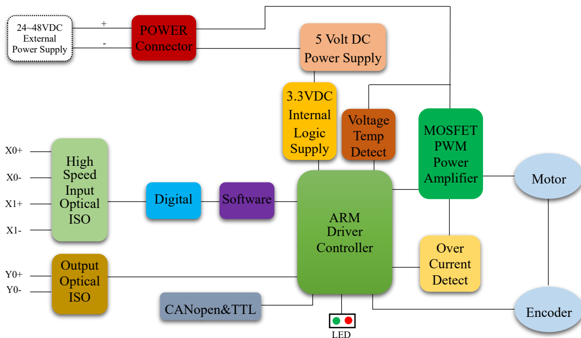
IR42EC Block Diagram
