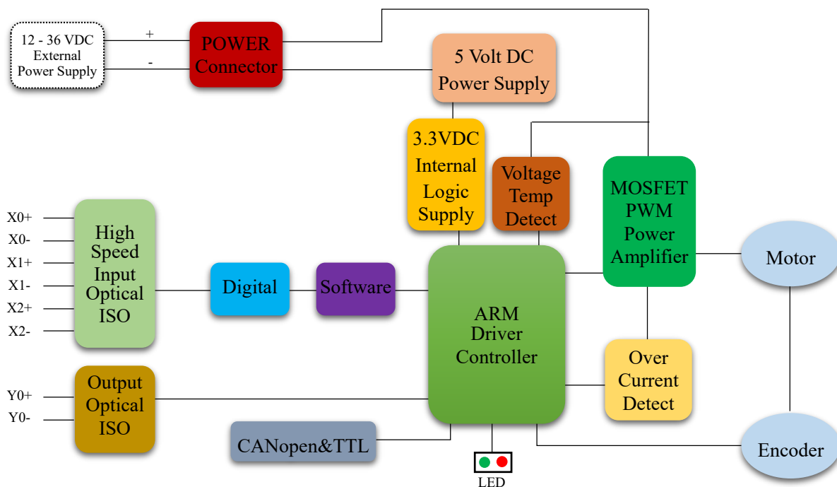
IR35EC Block Diagram
