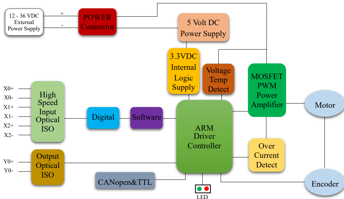
IR28EC Block Diagram
