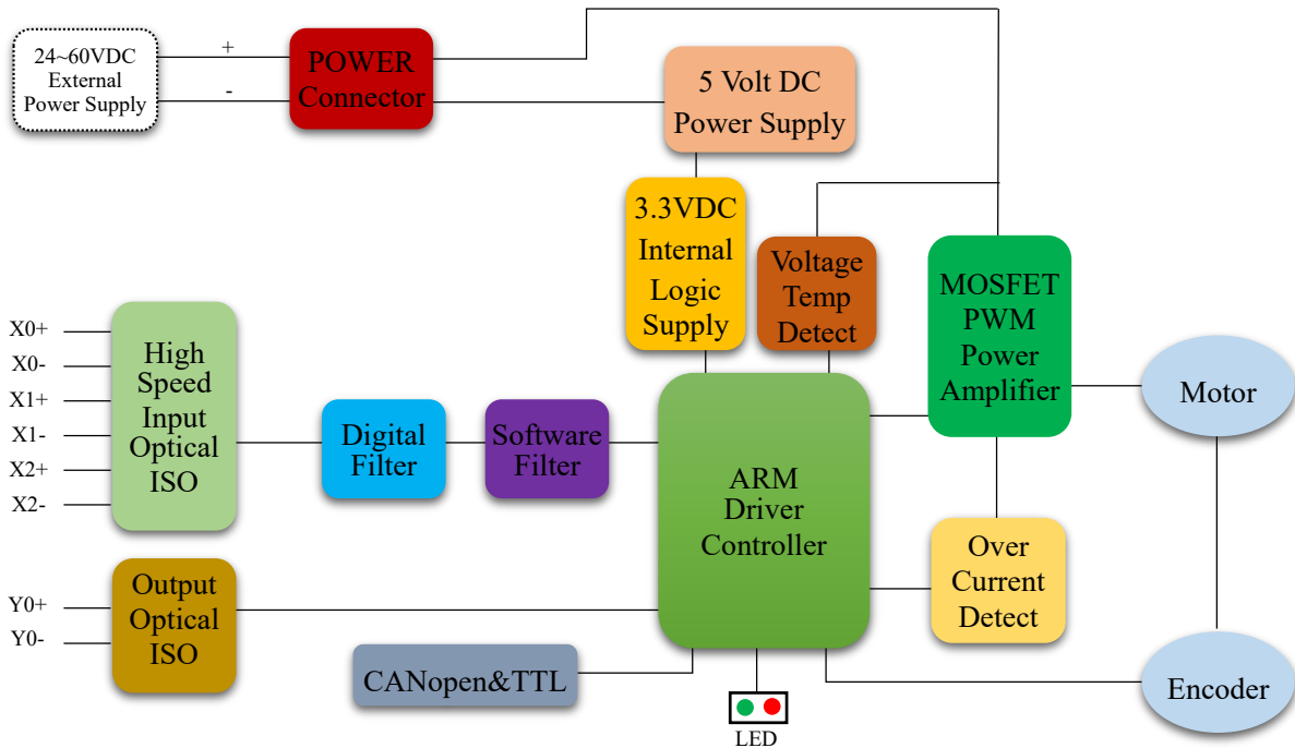
IH60EC Block Diagram
