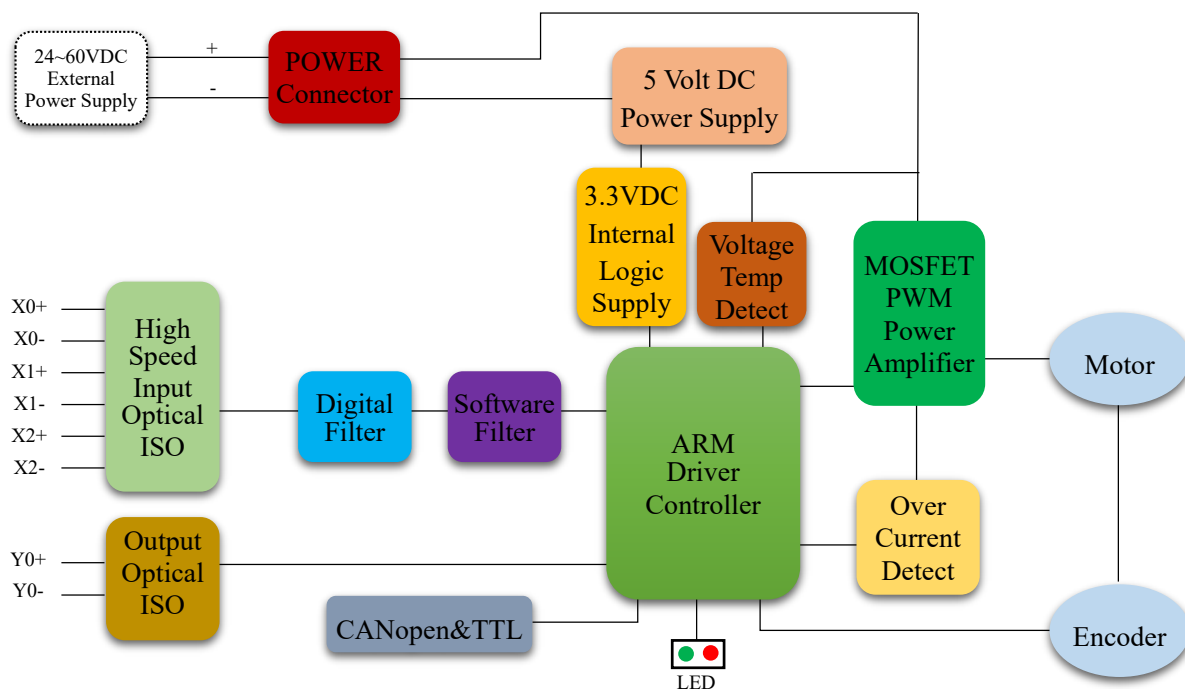
IH57EC Block Diagram
