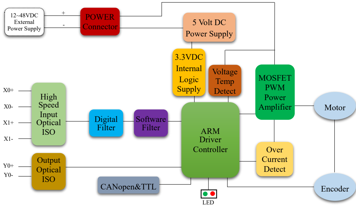
IH42EC Block Diagram
