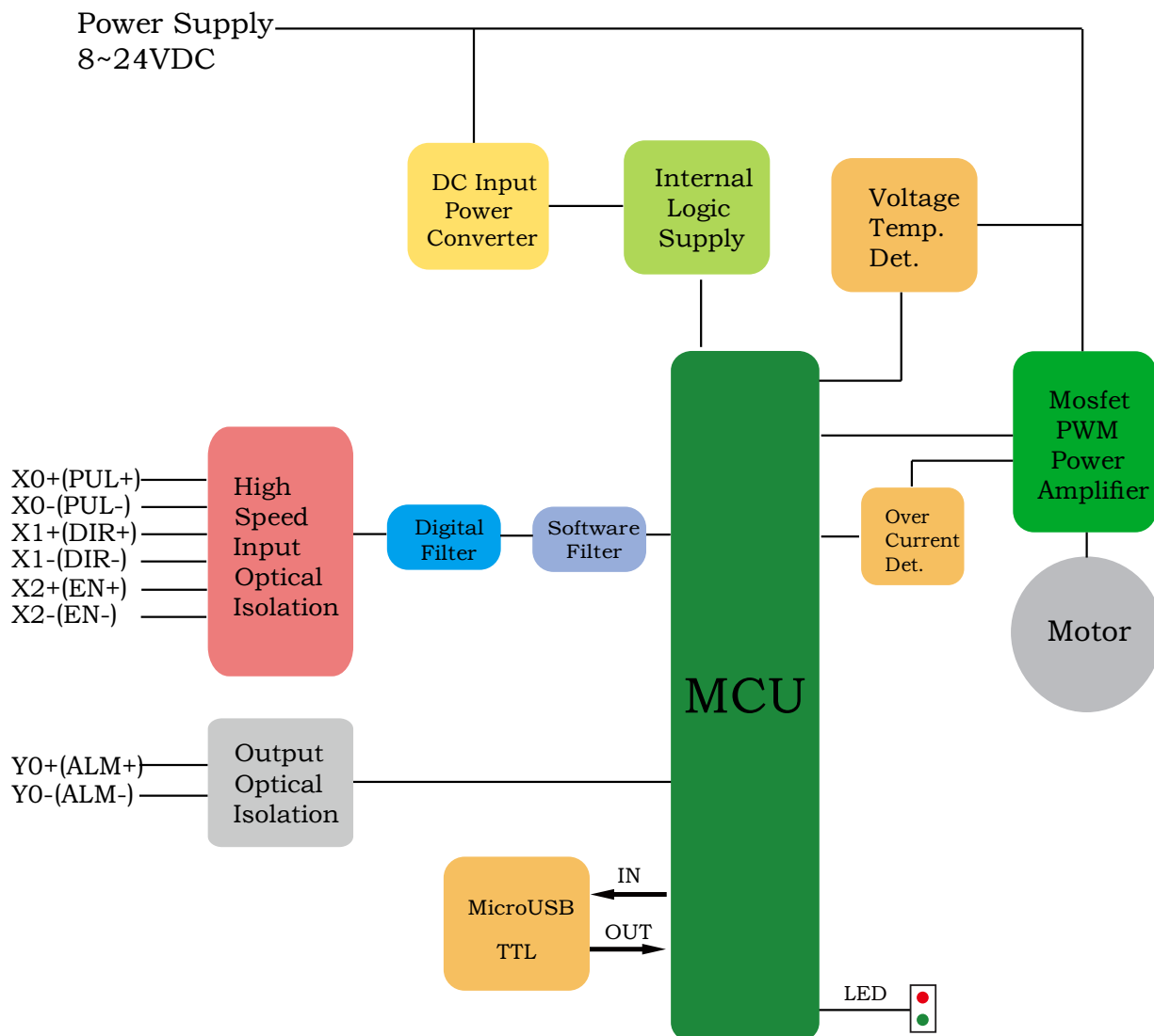
IR20E Block Diagram
